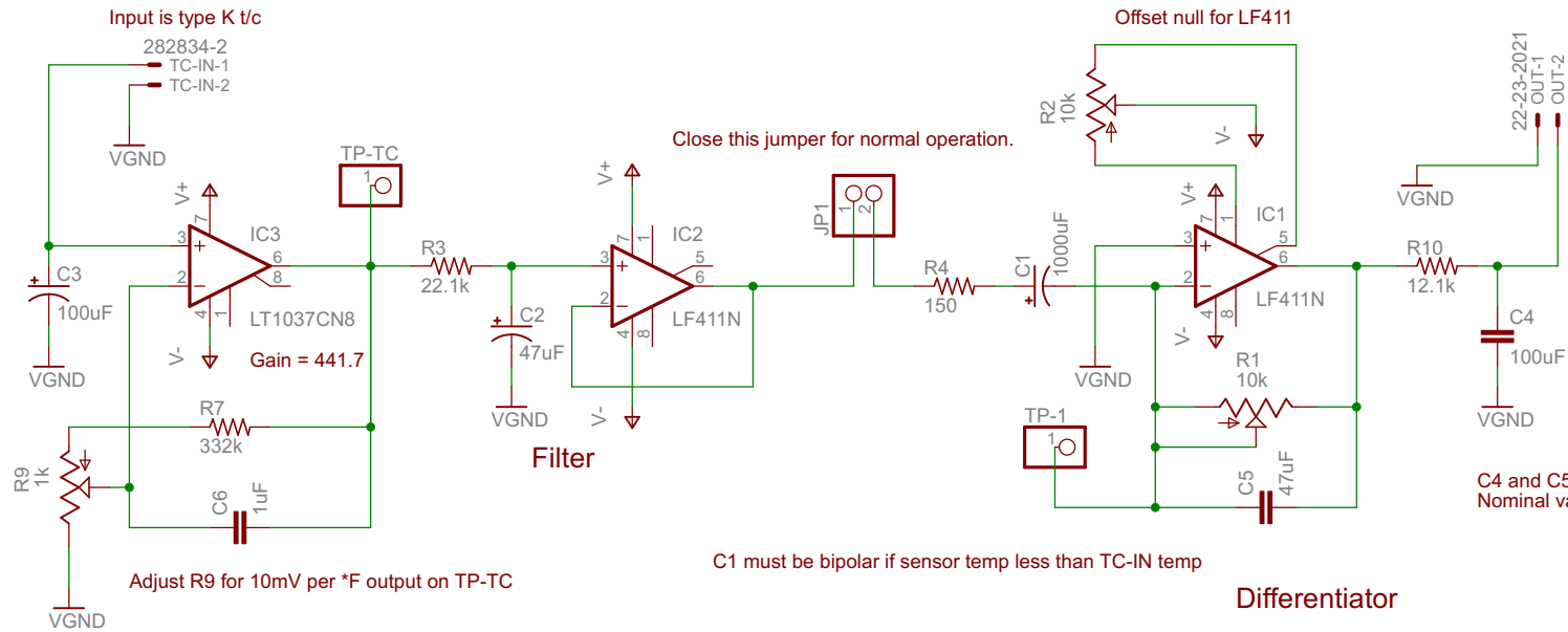
Thermocouple amp
